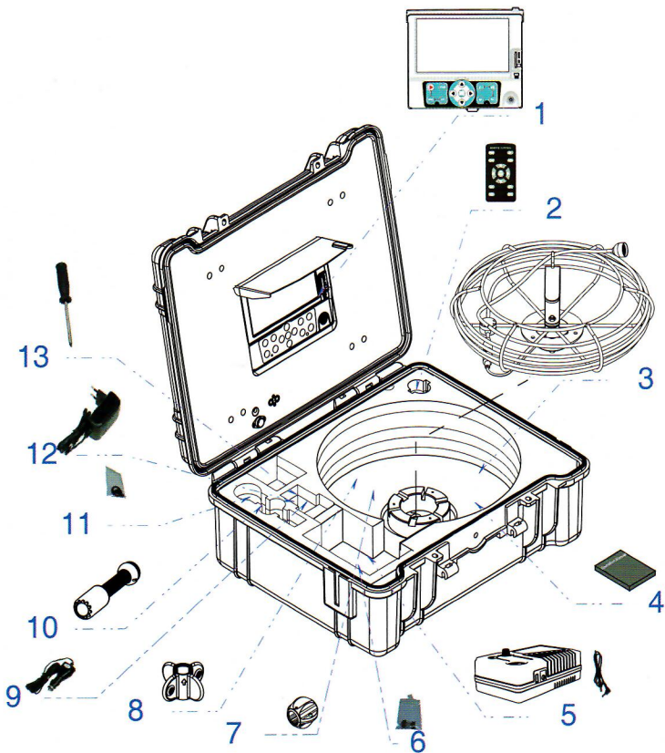
Figure 6. Package Contents
